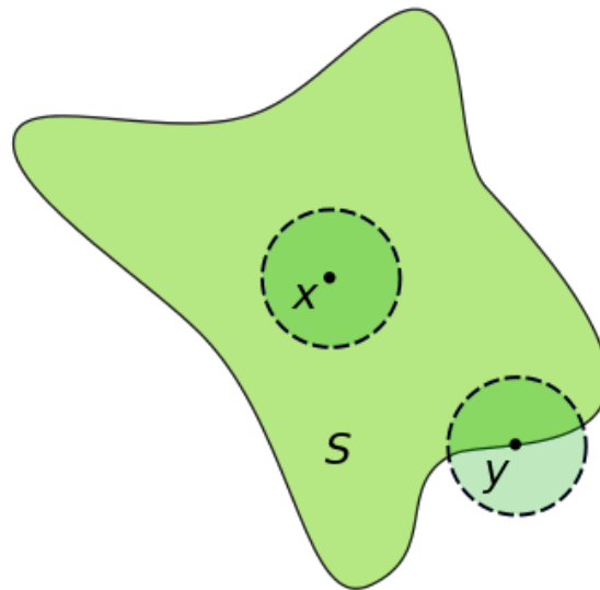
Figure 13.3: Inner points v.s. boundary points. Source: https://en.wikipedia.org/wiki/Interior_(topology)
