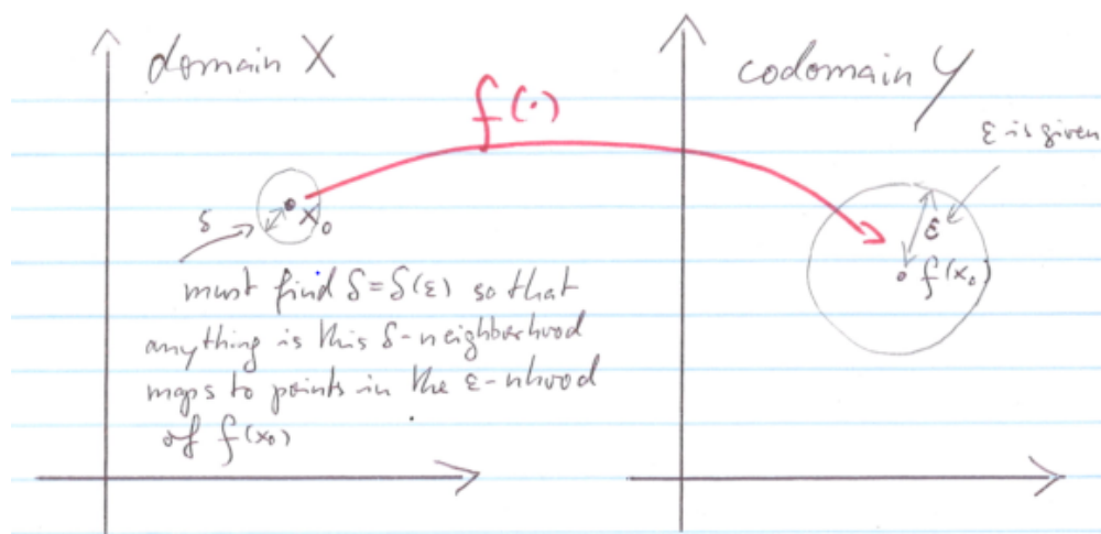
Figure 13.6: \varepsilon - \delta continuity
