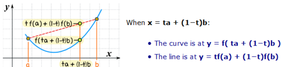
Figure 14.1: Convex function
