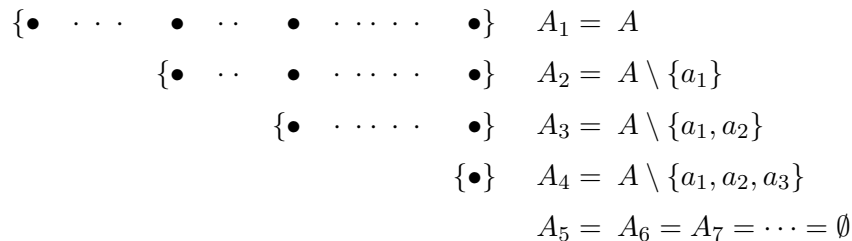
Figure 7.1: K = 4 : a_4 = \max(A) .
