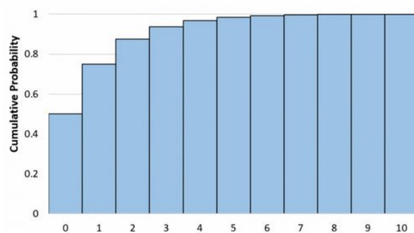
9.2 (Figure). CDF for \text{geom}(0.5) . 100
