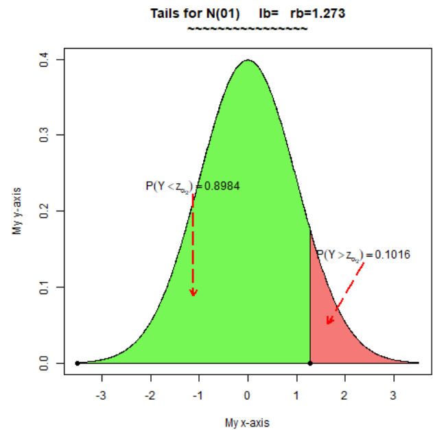
13.3 (Figure). (b) right tail area > 10%.
